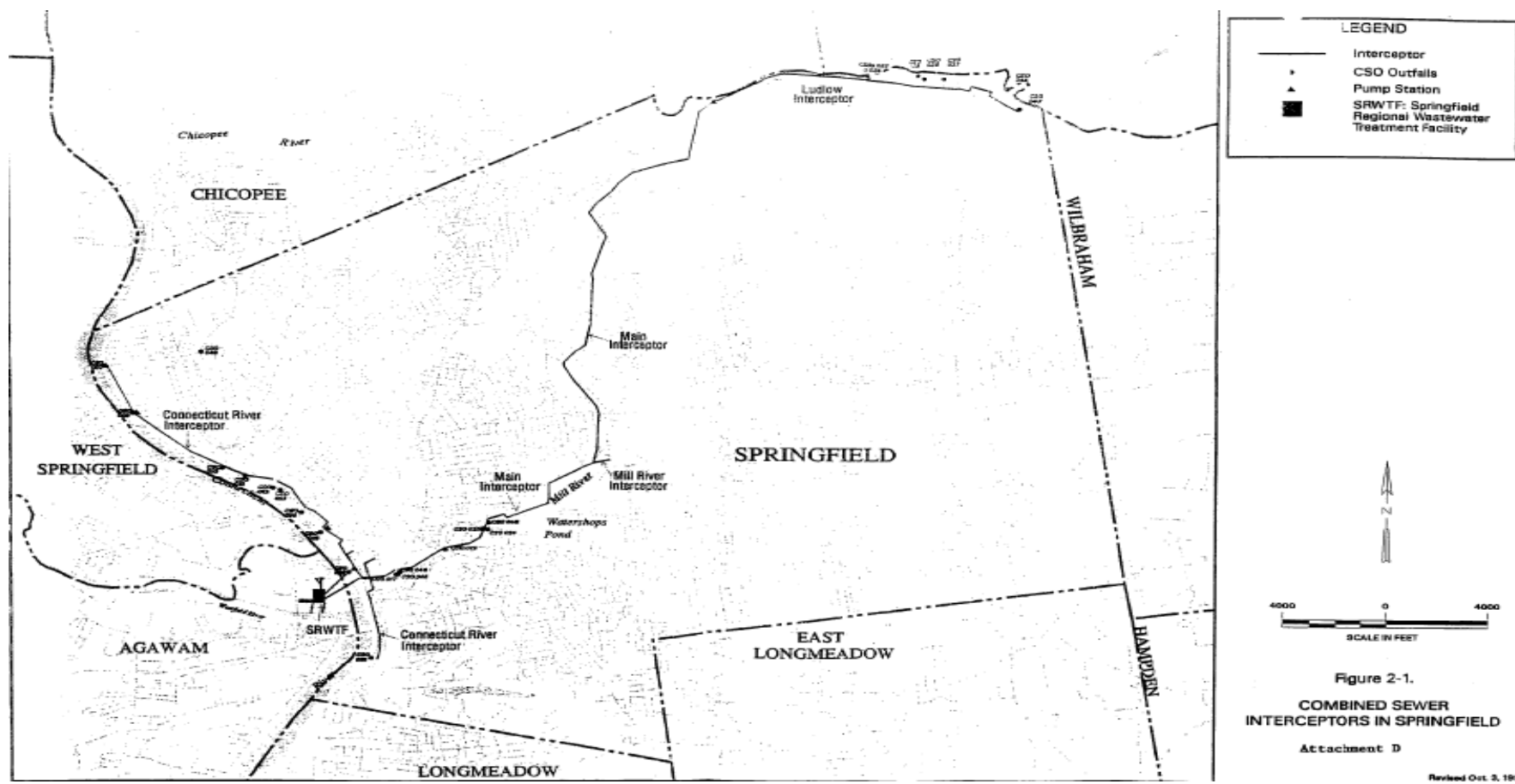
Figure 2: Combined Interceptor Sewers
